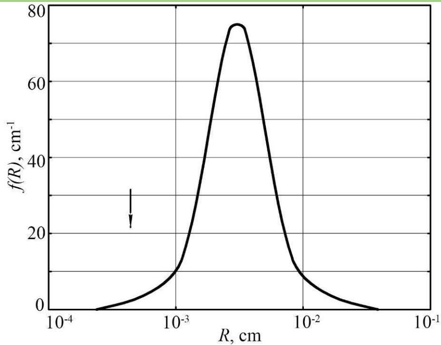
Fig. 3. The gas bubble size distribution function
